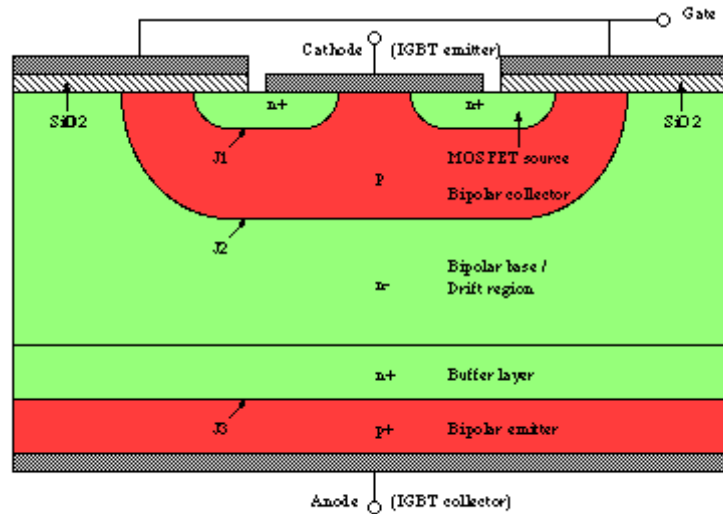
Fig.1: A typical IGBT structure
